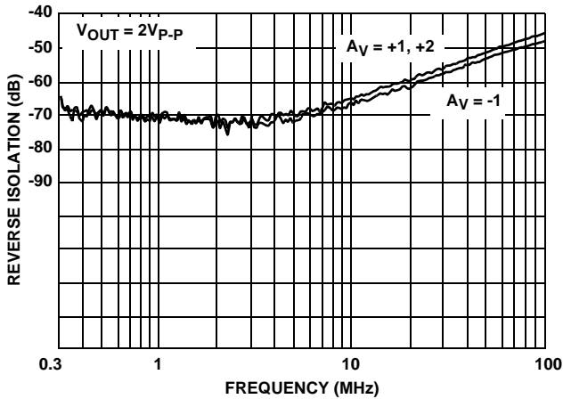
FIGURE 21. REVERSE ISOLATION
