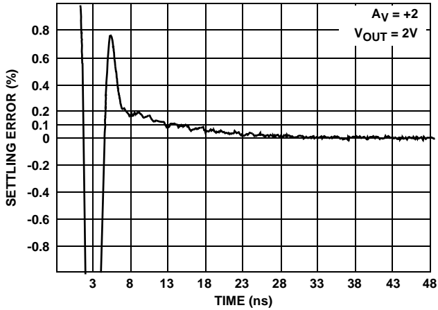
FIGURE 23. SETTLING RESPONSE
